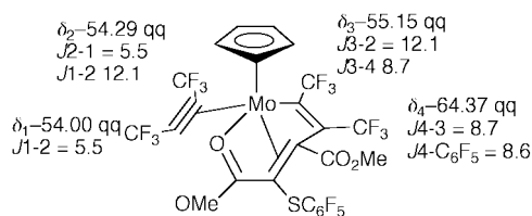
Fig. 2 The ^{19}\text{F} NMR assignments for [\text{Mo}\{\eta^4\text{-C}(\text{CF}_3)=\text{C}(\text{CF}_3)\text{-C}(\text{CO}_2\text{Me})=\text{C}(\text{CO}_2\text{Me})(\text{SC}_6\text{F}_5)\}(\text{CF}_3\text{C}\equiv\text{CCF}_3)(\eta^5\text{-C}_5\text{H}_5)] 3 .
